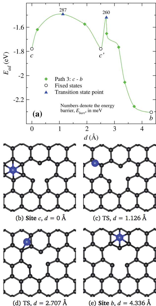
Fig. 9 (a) Minimum energy path for a Ni atom moving around the vacancy, from c to b . The x -axis represents the distance between the initial and final states. Open symbols stand for our static calculations while the solid ones are for results from cNEB results. In the middle and lower panels, Insets (b) to (e) show the positions of the atoms at some points marked in inset (a), where, the transition states (TS) are clearly indicated.
