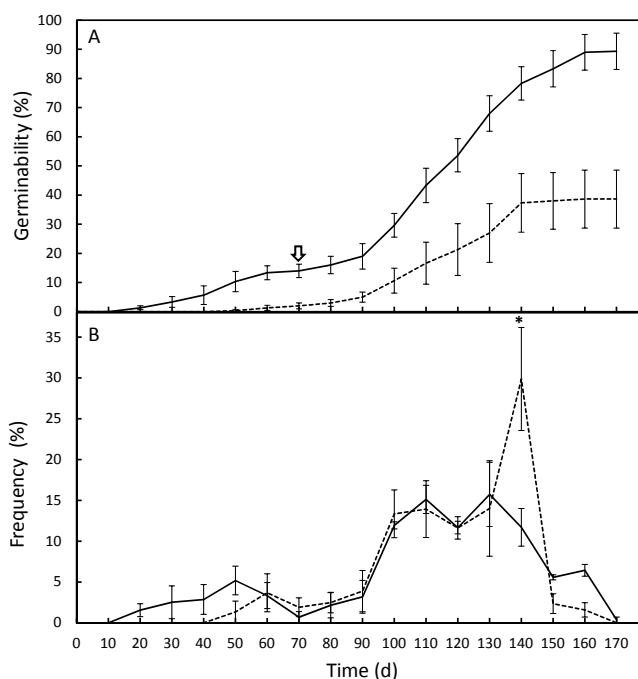
Figure 2. Photosynthetic photon flux density treatments (---PPFD81) and (—PPFD17) for Dioon edule seed germinability (A) and relative frequency of germination (B). The arrow indicates the beginning of significant differences between treatments P < 0.05 ; * significant differences P < 0.05 .
