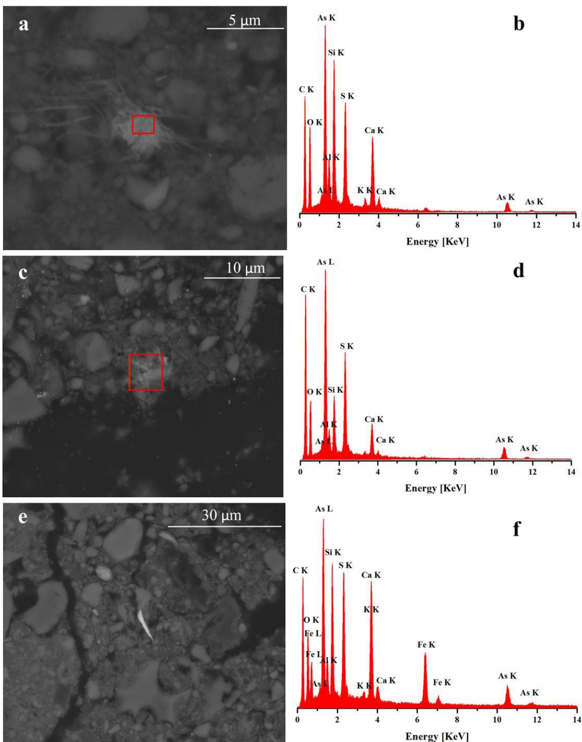
Figure 5. Backscattered SEM images of samples A (a and b), B (c and d) and D (e and f) showing diagenetic needle-like minerals commonly found in sediments of the contaminated spring (brighter areas indicate zones of higher atomic number).
