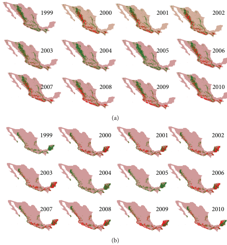
FIGURE 3: Incidence of wildfires in forest (a) and in rainforest (b). Green areas represent the polygon of the vegetation type and the red points symbolize the hot spots.
