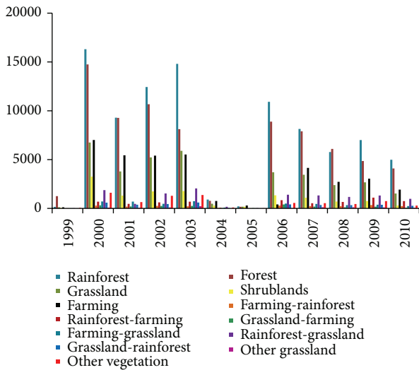
FIGURE 4: Time series of the yearly number of hot spots (wildfires) per vegetation type.
