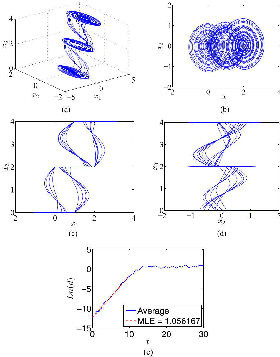
FIG. 5. Triple scroll attractor for the initial condition (0, 0, 0) in (a) the space (x_1, x_2, x_3) and its projections onto the planes: (b) (x_1, x_2) , (c) (x_1, x_3) , and (d) (x_2, x_3) . In (e), the largest Lyapunov exponent.
