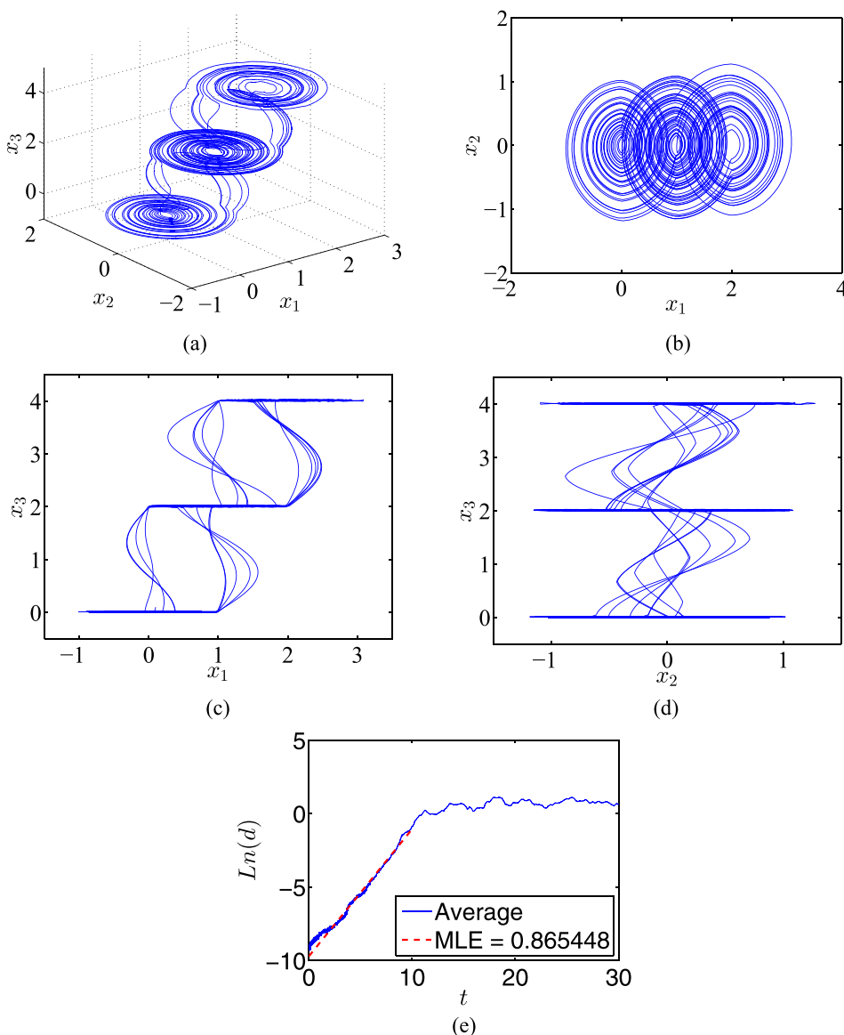
FIG. 6. Attractor of the system (21) with A given in (22) for the initial condition (0.1, 0.1, 0.1) in (a) the space (x_1, x_2, x_3) and its projections onto the planes: (b) (x_1, x_2) , (c) (x_1, x_3) , and (d) (x_2, x_3) . In (e), the largest Lyapunov exponent.
