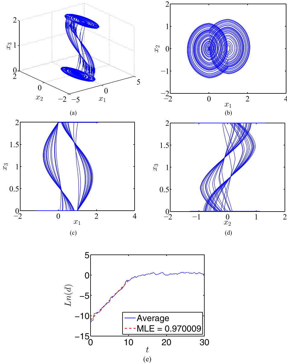
FIG. 4. Attractor of the system (15) with A and V given in (14) for the initial condition (0, 0, 0) in (a) the space (x_1, x_2, x_3) and its projections onto the planes: (b) (x_1, x_2) , (c) (x_1, x_3) , and (d) (x_2, x_3) . In (e), the largest Lyapunov exponent.
