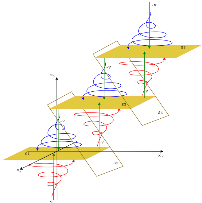
FIG. 3. A mechanism to generate a triple-scroll chaotic attractors without equilibria.
