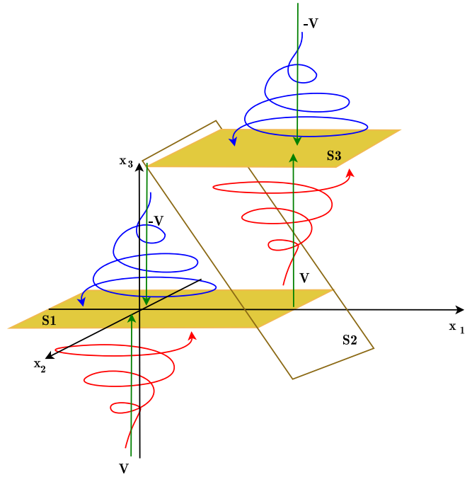
FIG. 2. A mechanism to generate a double-scroll chaotic attractors without equilibria.
