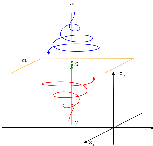
FIG. 1. A “saddle-focus like” locate at the point Q = (-k_1, -k_2, \tau) .
