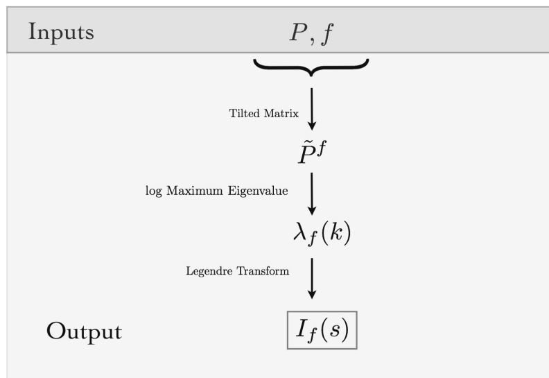
Figure 3. Algorithmic view of the method: Inputs are the maximum entropy Markov transition matrix and a feature. From the inputs, the tilted transition matrix can be built. The rate function of the feature is obtained as the Legendre transform of the log maximum eigenvalue of the tilted transition matrix. Using this framework, we can estimate the large deviations of the average values of the features.
