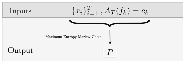
Figure 2. Algorithmic view of the maximum entropy Markov chains (MEMC): Inputs are the spike trains \{x_i\}_{i=1}^T and the average values of a set of features. The output is the MEMC transition matrix P .
