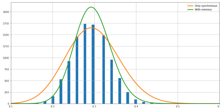
Figure 8. The fluctuations of the synchronous feature around the mean computed from the sample of the Markov chain are indicated with the bars. The Gaussian fluctuations around the mean predicted by the large deviations rate functions of both models are plotted. The curve predicted by the Markov model obtained from \mathcal{H} is in green and the curve predicted by the model obtained from \tilde{\mathcal{H}} is in orange.
