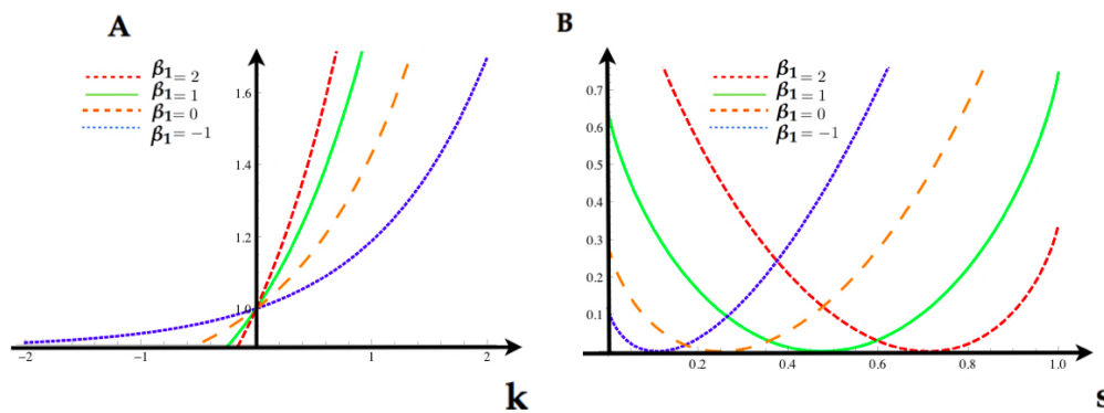
Figure 4. (A) Scaled cumulant generating function (SCGF) (Equation (24)) for the feature f_1 of the first example computed at the values provided by the table above. (B) Rate function for the same feature computed at the same parameter values as the SCGF. Each of these functions are obtained taking the Lagrange transform of the respective SCGF in (A).
