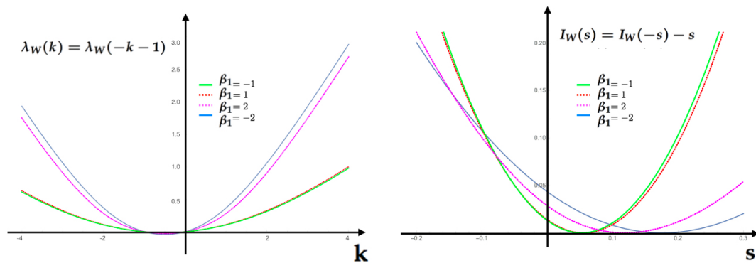
Figure 5. Gallavotti–Cohen symmetry relationship for the information entropy production IEP for values in Table 1. Left SCGF \lambda_W(k) . Right rate function of the IEP feature W , I_W(s) .
