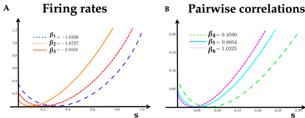
Figure 6. (A) Rate functions for the firing rates of each neuron of the Ising model. The minimum of the rate functions coincide with the expected value of the firing rates in Table 2. (B) Rate functions for the pairwise interactions computed from the parameters in Table 2.
