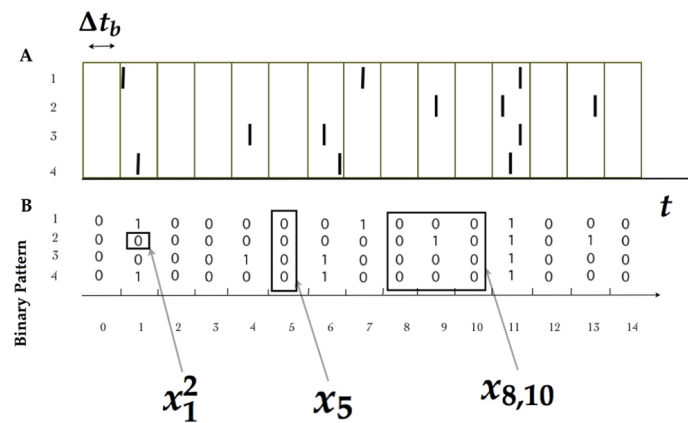
Figure 1. (A) Each bar indicates a spike of a neuron indexed from 1 to 4 in continuous time. (B) After binning \Delta t_b , the spiking activity is transformed into binary patterns in discrete time. We illustrate the notation used throughout this paper.
