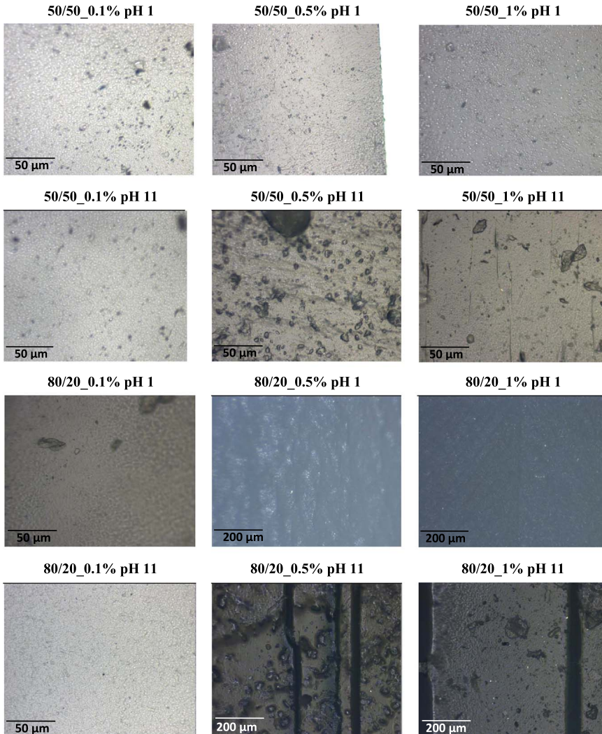
Fig. 9. Images of selected PMMA/PU/CePO 4 IPNs.
