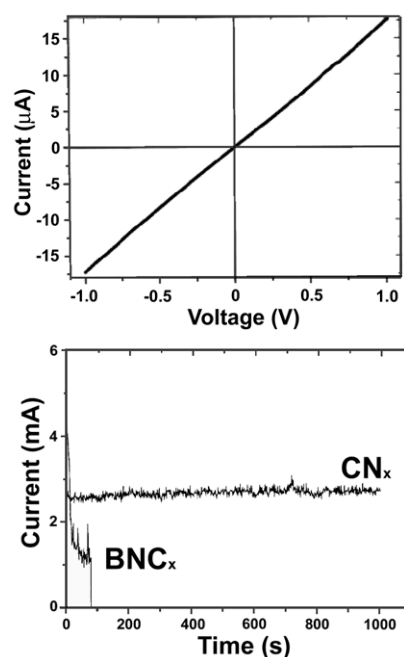
Fig. 10 (a) I-V characteristics of a rope of N-doped MWNTs. The rope displays stable field emission and a marked low-resistance metallic behavior (linear I-V curve, R \sim 70 K). (b) Plot of the field-emission stability of N-doped MWNT CN x compared to BNC x ( x < 0.1 ). CN x nanotube film emission is stable at low and high current densities. Note that BNC x nanotubes do not show stable electron emission 70 . (Reprinted with permission from 70 . © 2003 Springer-Verlag.)
