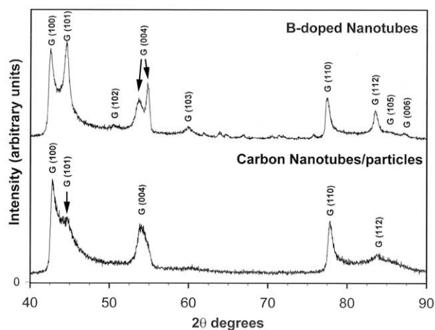
Fig. 5 XRD patterns from the inner core deposits obtained from BN/graphite arc discharge experiments compared with pure MWNTs and nanoparticles. The pattern from 40–90 2\theta degrees clearly shows the high degree of crystallinity of the B-doped sample [note the (101), (103), and (112) reflections that denote three-dimensional order and ABAB stacking of the layers]. Also note that the (001) reflection exhibits two peaks corresponding to 3.35 Å and 3.42 Å, thus confirming the presence of two different 'graphitic' structures (graphite-like ABAB... possibly from faceted areas of polygonized nanotubes and turbostratic graphite arising from concentric graphene cylinders, MWNTs).
