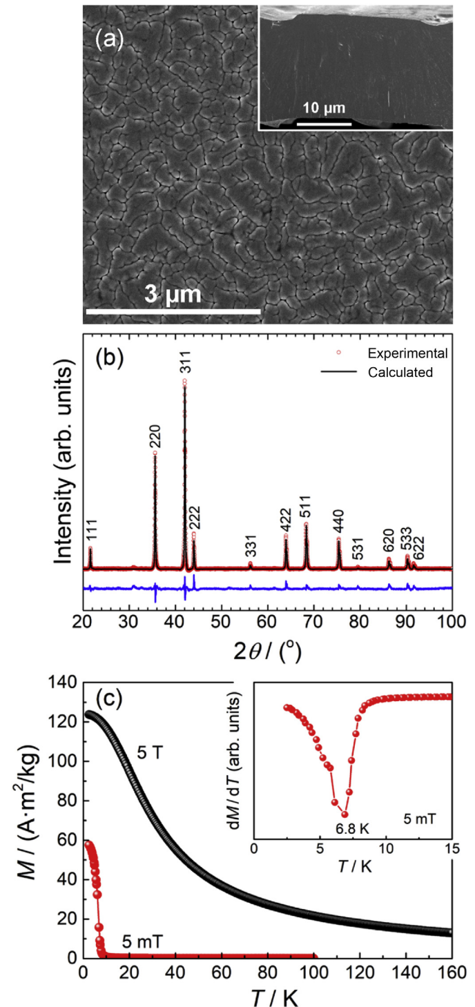
Fig. 1. (a) SEM micrographs showing the ribbon free surface (foreground image) and cross-section (inset); (b) Experimental and Le Bail refinement (Bragg R -factor of 0.692) of the room temperature X-ray power diffraction of melt-spun ribbons; (c) Temperature dependence of the specific magnetization determined under low (5 mT; full red symbols) and high (5 T; full black symbols) magnetic fields. Inset: dM/dT curve at 5 mT; the Curie phase transition temperature T_C appears at 6.8 K.
