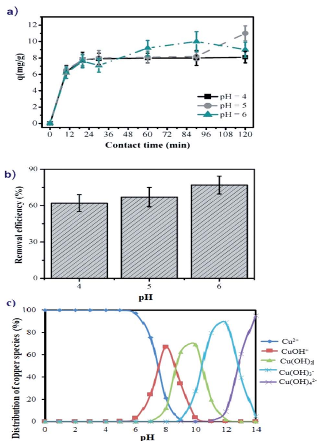
Fig. 4 Adsorption of Cu(II) ions on the manganite surface showing the influence of: (a) the contact time at different pH values; (b) pH of solution at 1 h of contact time and (c) copper species distribution in aqueous solution (modelling with visual MINTEQ 3.1 software, for 25 mg L -1 of copper at 1 atm and 25 °C). The initial copper concentration is 25 mg L -1 .
