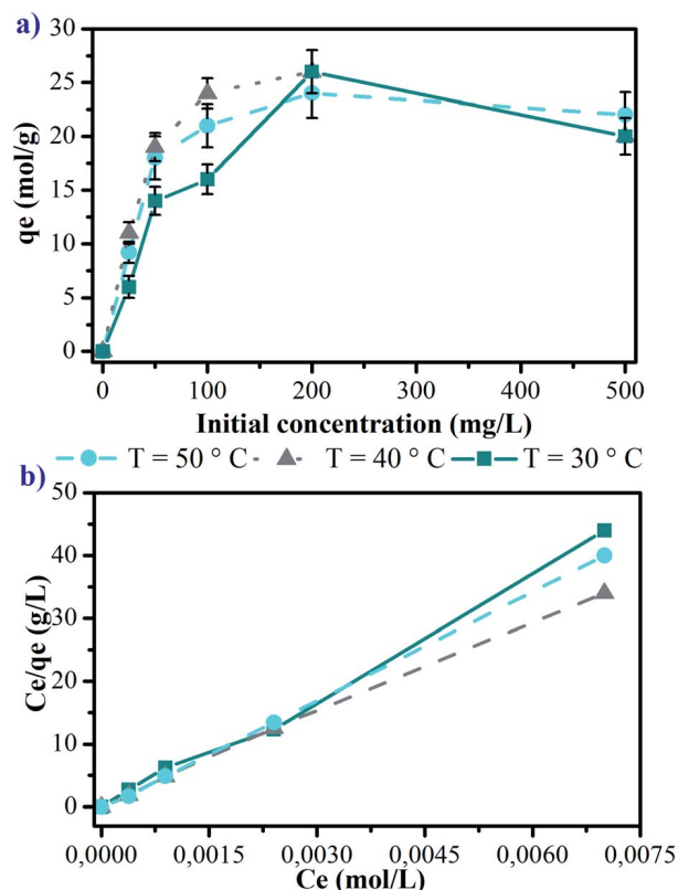
Fig. 5 Influence of the initial concentration of Cu(II) ions and the temperature on the adsorption on manganite: (a) adsorption isotherms at contact time of 24 hours and (b) linear shape of the adsorption isotherms.
