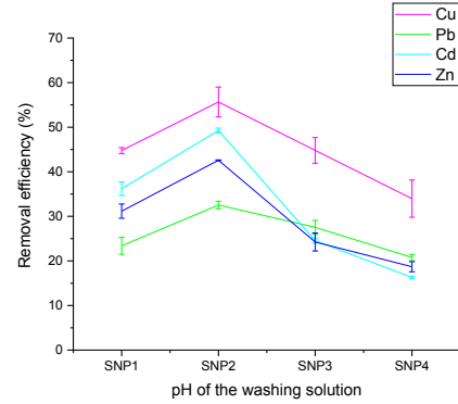
Fig 2. Effect of SN and SH pH on the removal of heavy metals from soils (Soil-solution ratio = 40, time is 6 hr concentration = 3). Each point is the average of triplicate samples. SNP1 = 3; SNP2 = 4; SNP3 = 5; SNP4 = 6; SHP1 = 3; SHP2 = 4; SHP3 = 5; SHP4 = 6.
