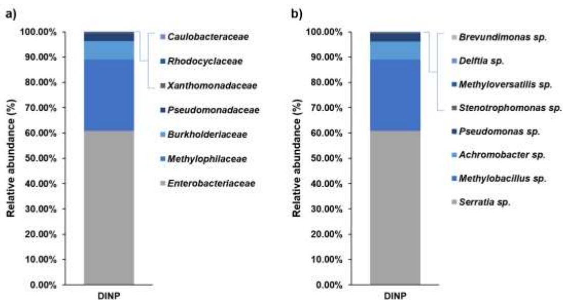
Figure 1. Identification of the bacterial diversity of the SSB-consortium. (a) at family level; (b) at genus level.
