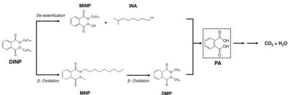
Figure 6. Proposed pathways for DINP degradation by the SSB-consortium. The dotted box indicates that the metabolite was not detected in this study.
