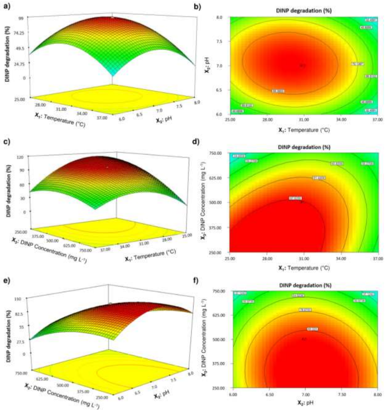
Figure 2. Contour and 3D response surface plots showing the influence of pH, temperature, and initial DINP concentration on the % of DINP biodegradation by the SSB-consortium.
