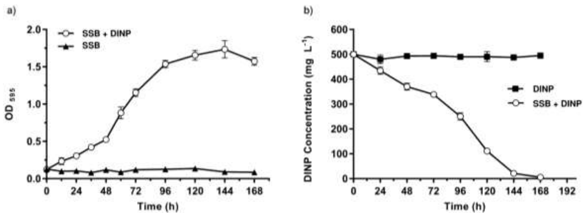
Figure 3. Growth of the SSB-consortium and DINP biodegradation kinetics started at 500 mg L -1 DINP: a) Evaluation of cell growth in MSM with or without DINP as the only carbon source, and b) degradation of DINP by the SSB-consortium under optimal conditions (31 °C, pH 7 and 500 mg L -1 ) in MSM. Non-inoculated MSM was employed as control (black squares). Error bars indicate the standard error of the three replicates.
