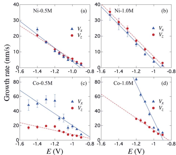
Fig. 4 Variation of the metallic layer and NWs average growth rates V_x (triangles) and V_z (circles) for \mu HGPs grown using the (a) Ni-0.5 M, (b) Ni-1.0 M, (c) Co-0.5 M and (d) Co-1.0 M electrolytes as function of the reduction potential E . The continuous and dotted lines are linear fits to the data and error bars correspond to one standard deviation obtained from the different \mu HGPs of a same sample.
